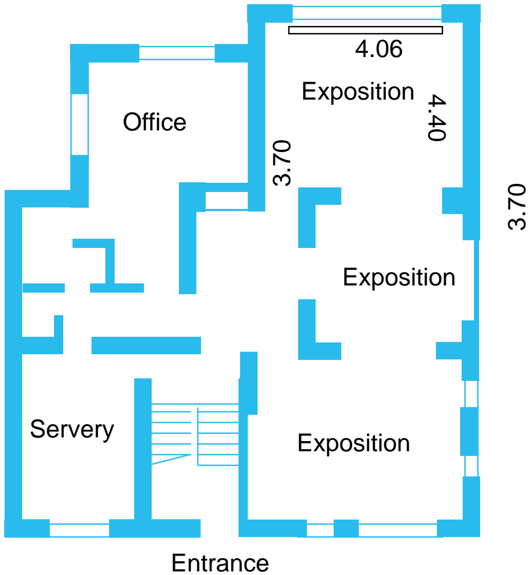
Assar art gallery floor plan SC 1:100
